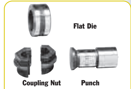
TYPICAL 20 TON STYLE TOOLING
